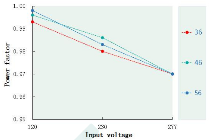
Power factor VS Input voltage(DL-240W-V56A/P/X-MXG)
