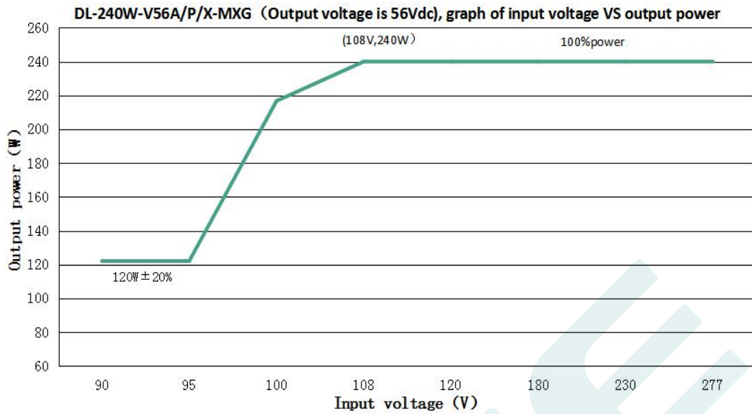
DL-240W-V56A/P/X-MXG (When the output voltage is 56Vdc, the rated output current value and output power corresponding to different input voltage)
